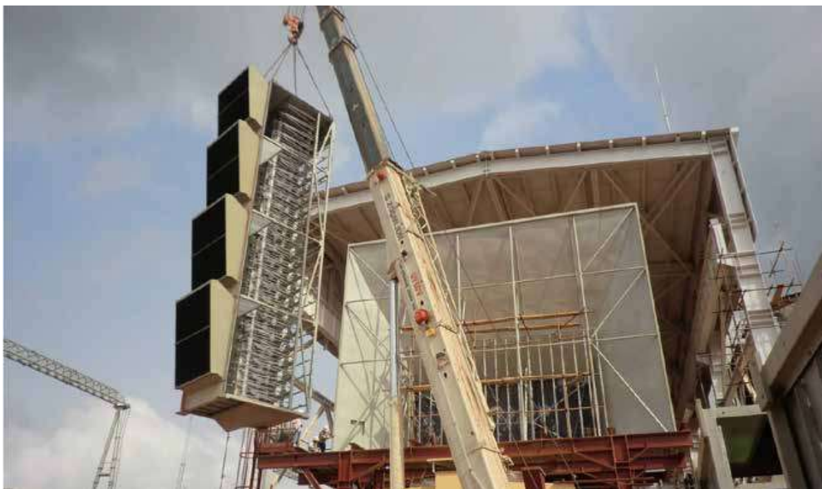
尼日利亚欧莫托休二期燃机电站项目 Omotosho Phase II 500mw Open Cycle Power Plant Project in Nigeria
